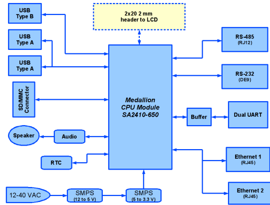
Gateway 2 Block Diagram
